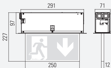
RECESSED CEILING INSTALLATION (DISPLAY 3000/G6)
