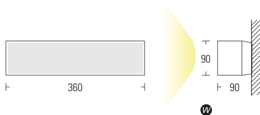
Wandmontage
